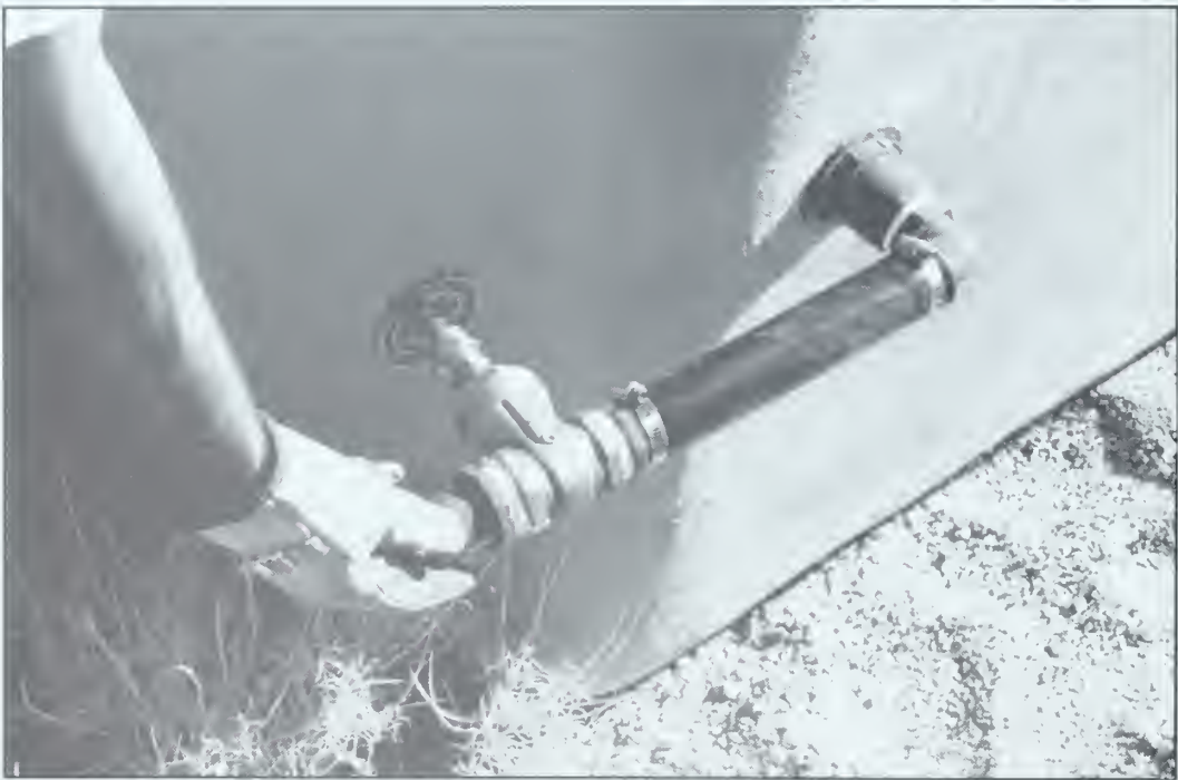
Photo 5. Completed/installed plumbing unit for big game guzzler.
